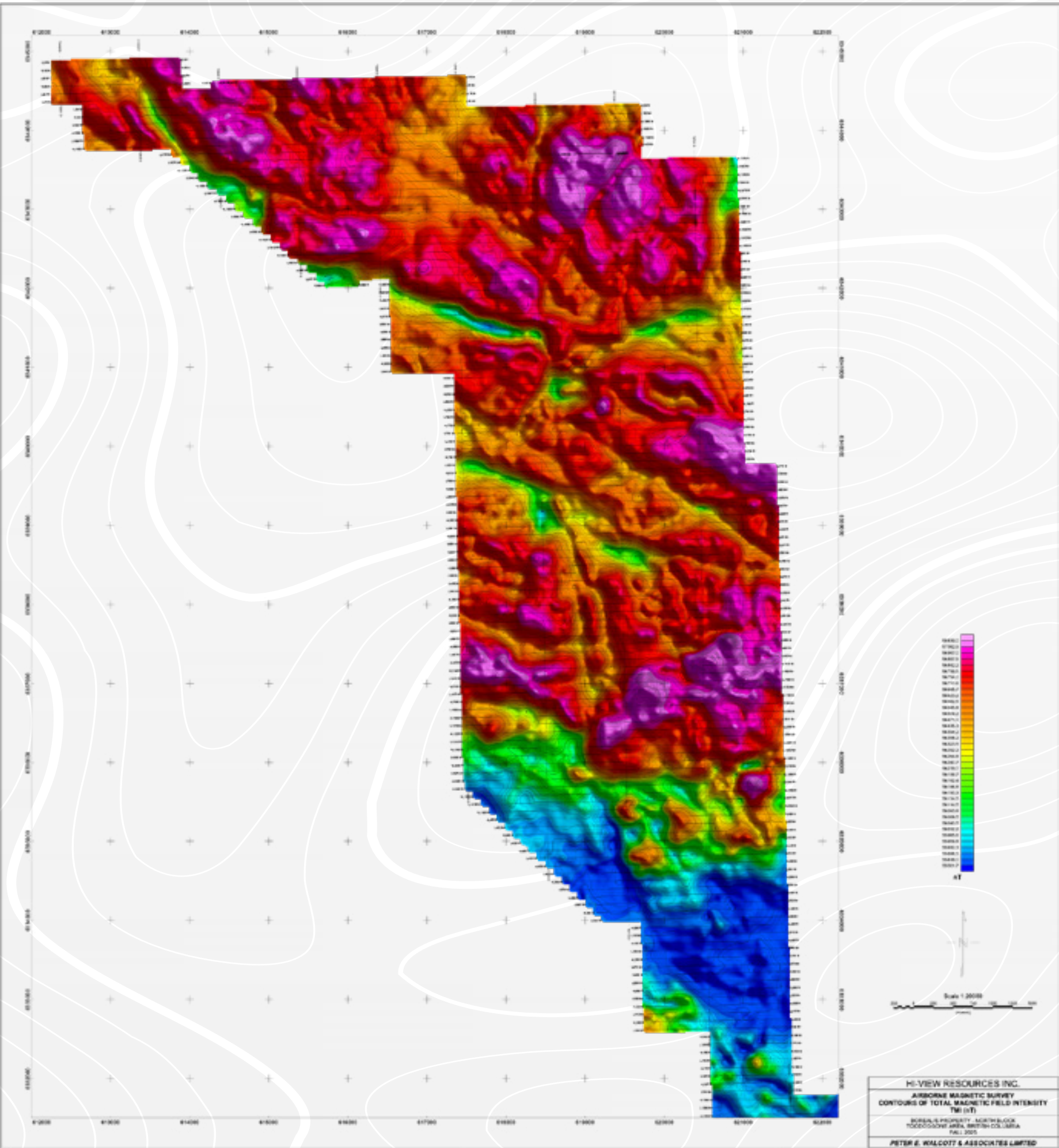
AIRBORNE MAGNETIC SURVEY CONTOURS OF TOTAL MAGNETIC FIELD INTENSITY TMI (nT)
