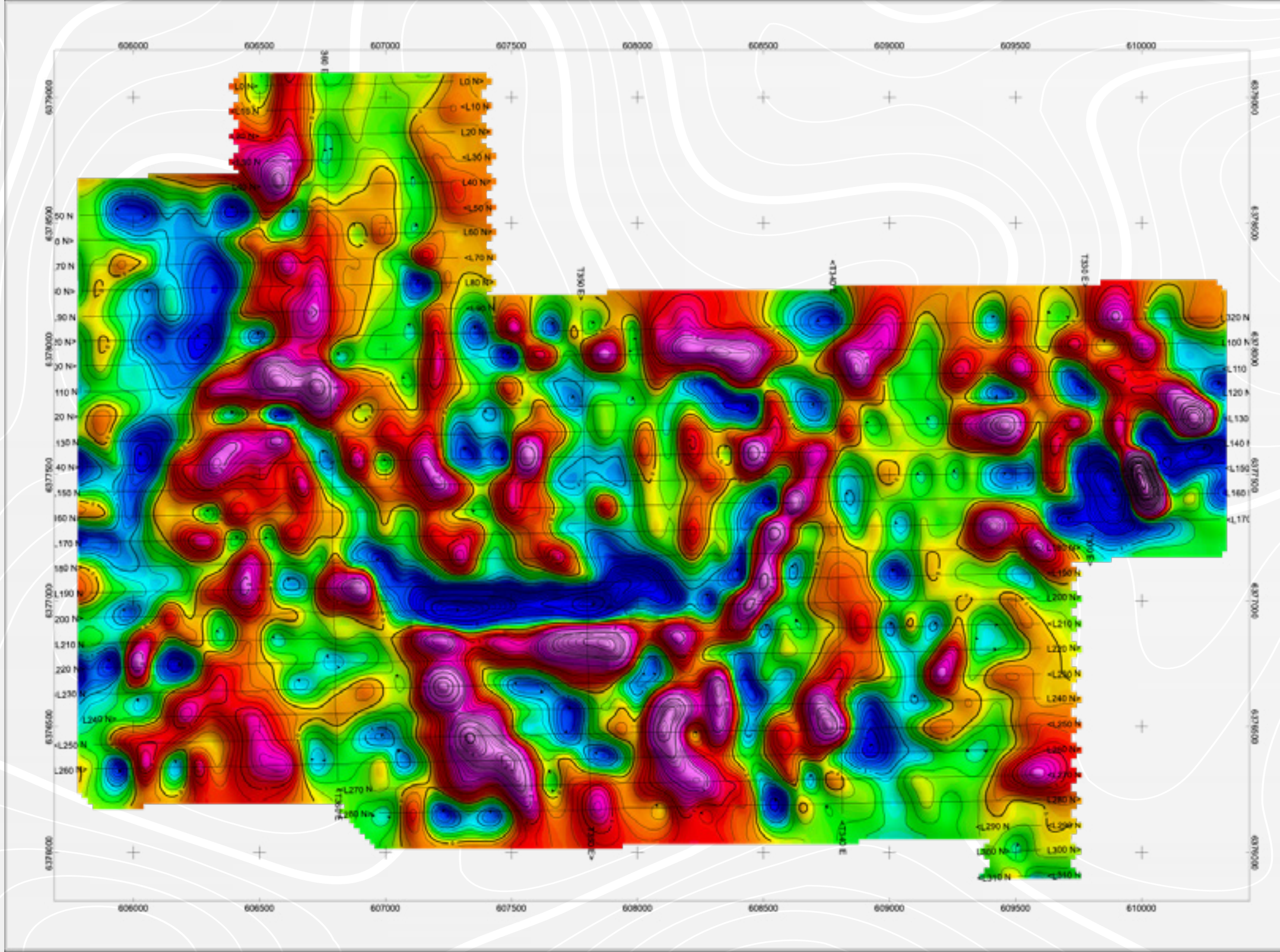
AIRBORNE MAGNETIC SURVEY CONTOURS OF CALCULATED IVD (nT/m)
