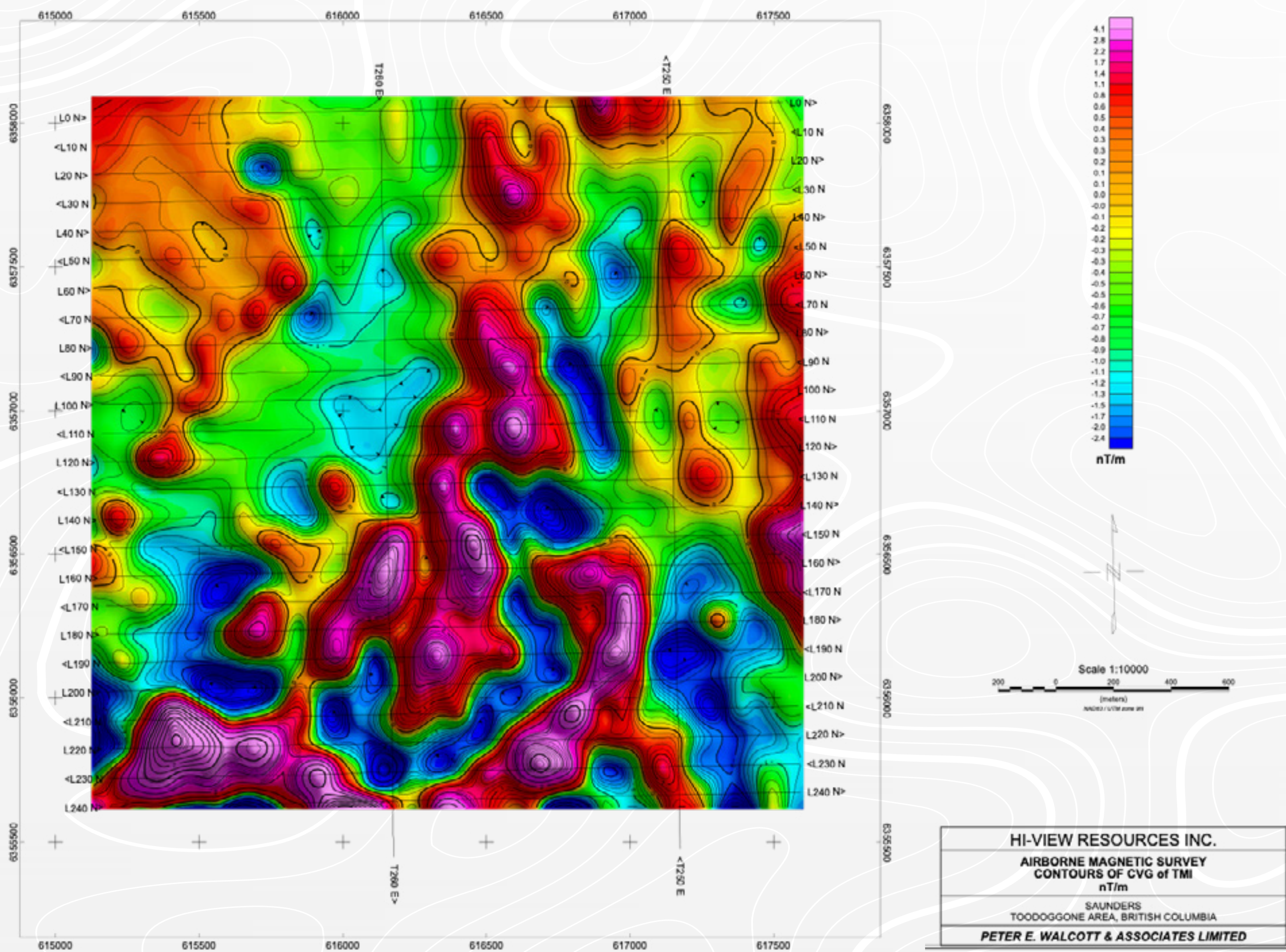
AIRBORNE MAGNETIC SURVEY CONTOURS OF TOTAL MAGNETIC FIELD INTENSITY TMI (nT)
