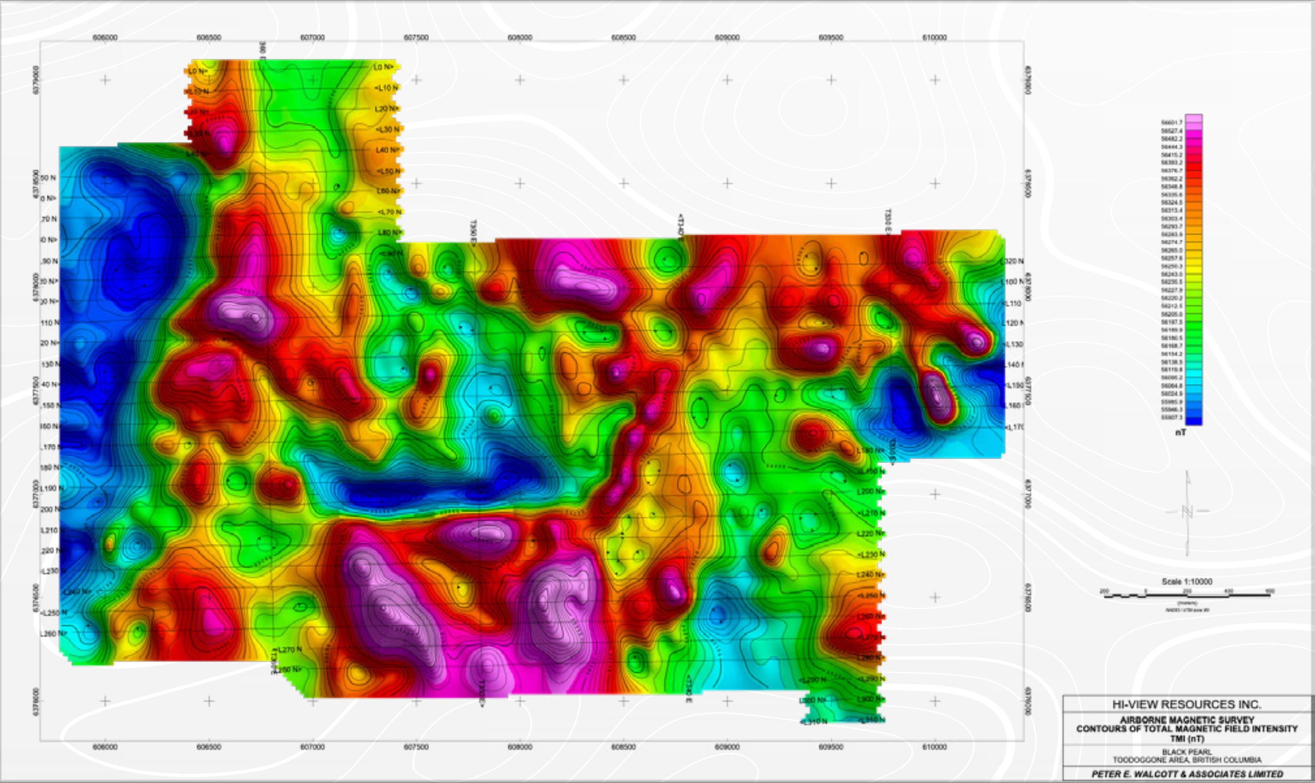
AIRBORNE MAGNETIC SURVEY CONTOURS OF TOTAL MAGNETIC FIELD INTENSITY TMI (nT)
